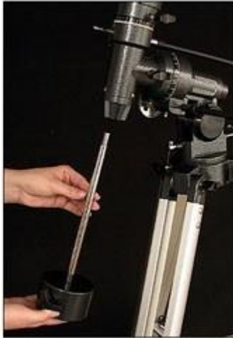
Figure 28 -- Attaching the balance shaft and counterweight to the equatorial mount.
